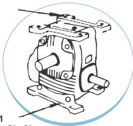
Foot Type 1 in position 2 (away from input Shaft)
